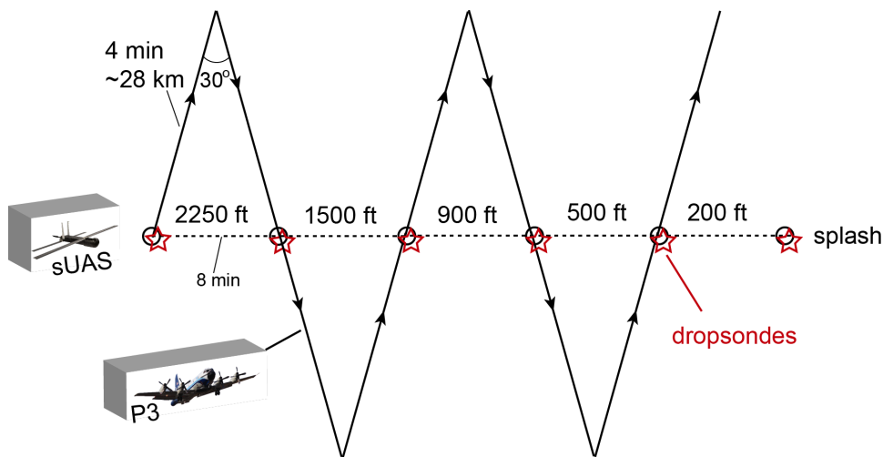
*Stepped descent inflow module of sUAS (with P-3)
