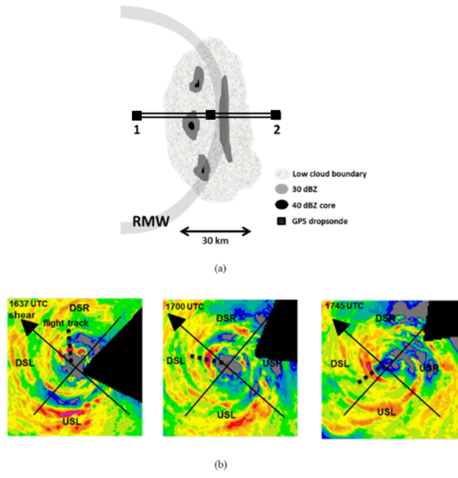
Figure CBMI: P-3 Convective burst module: (a) Radial penetrations / bowtie pattern. Black squares denote locations of GPS dropsondes from P-3. This pattern should be repeated multiple times as time allows, following the CB around the storm (or in place if the CB remains confined downshear). (b) Example of sampling strategy following CBs around the storm, beginning downshear right (DSR) and into the upshear quadrants. Each radial pass is separated by ~30 minutes.
