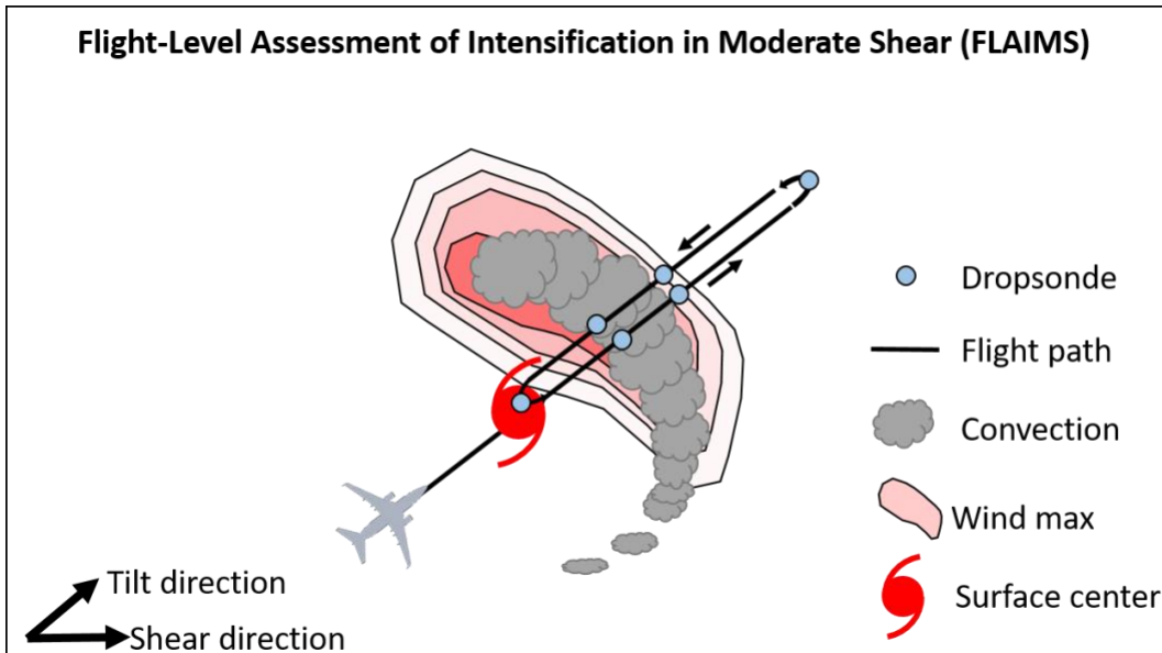
Figure 1: Schematic illustration of the FLAIMS module. In this example, the initial point of the module is the low-level vortex center, and an initial outbound leg is followed by an inbound leg along the same azimuth where the maximum flight-level winds are found. Following this inbound leg and center penetration, the plane turns around at the vortex center location and begins another outbound leg. This can be repeated for a total of 2–6 combined inbound and outbound legs. Note that the initial leg can alternately be inbound, and the module can either end with a center crossing or at the outer point.
