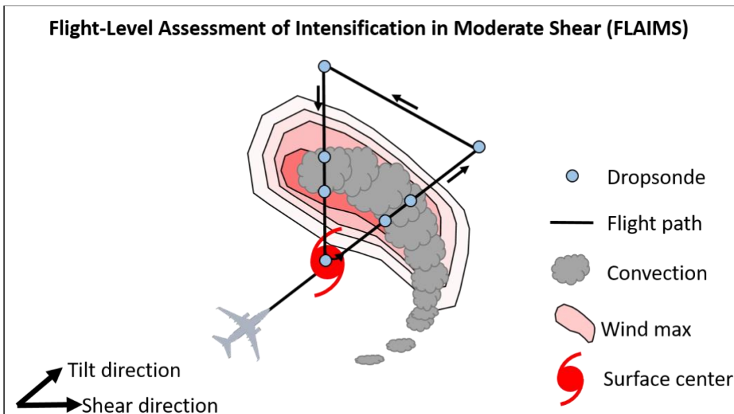
Figure 2: Schematic illustration of Pattern #2 for the FLAIMS module. In this example, the initial point of the module is the low-level vortex center, and an initial outbound leg is followed by a leg that flies 45 degrees downwind, and the triangle is then completed by flying inbound to the center. Following this inbound leg and center penetration, the plane turns around at the vortex center location and begins another outbound leg along the same azimuth as the initial outbound leg. This can be repeated multiple times.
