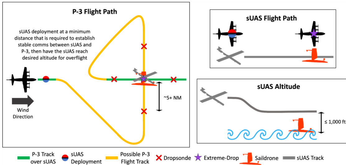
Fig. 5: P-3 and sUAS flight patterns for the saildrone overflight module. The sUAS is deployed far upwind (distance pending other variables) of the saildrone at the red/black/blue circle. The following goal would be to have the P-3 fly overhead the saildrone at the nearest time possible as the sUAS overflies the saildrone (depicted in green). The P-3 will (pending safety) deploy expendables ~5 NM either side of the saildrone and a deployment of all available types of expendables directly overhead the saildrone. During the time between the deployment of the sUAS and the overfly, the P-3 pattern depends on conditions, with the orange path depicting what would be preferred. The sUAS flight path (top right; gray) should be downwind directly to the saildrone. During this time, the sUAS will drop to \leq 1,000 ft (pending conditions) for the overflight. If battery and conditions permit the sUAS to circumnavigate the TC and overfly the saildrone again, then the final leg of the pattern is repeated (final green line).
